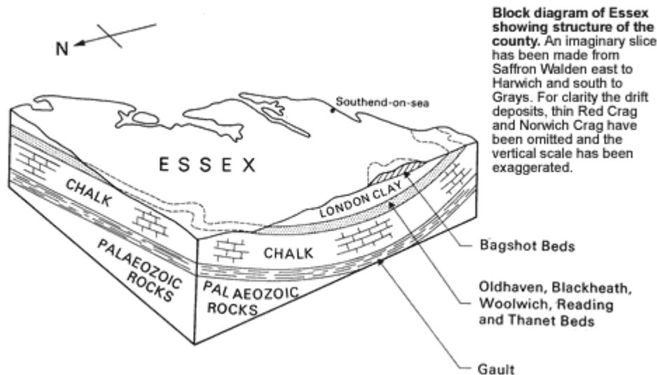
Figure 39: Structural Cross Section of Essex
