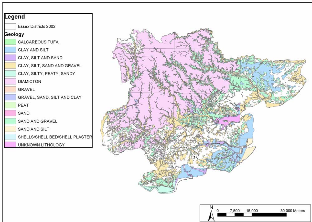
Figure 38: Surface Geology of Essex
