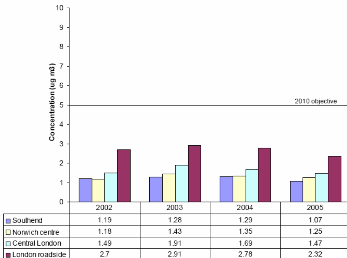
Figure 21: Annual Mean Concentrations of Benzene
